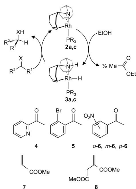
Scheme 2. Simplified catalytic transfer hydrogenation cycle by which substrates 4–8 are quantitatively converted into the corresponding alcohols with catalysts 2a,c .
