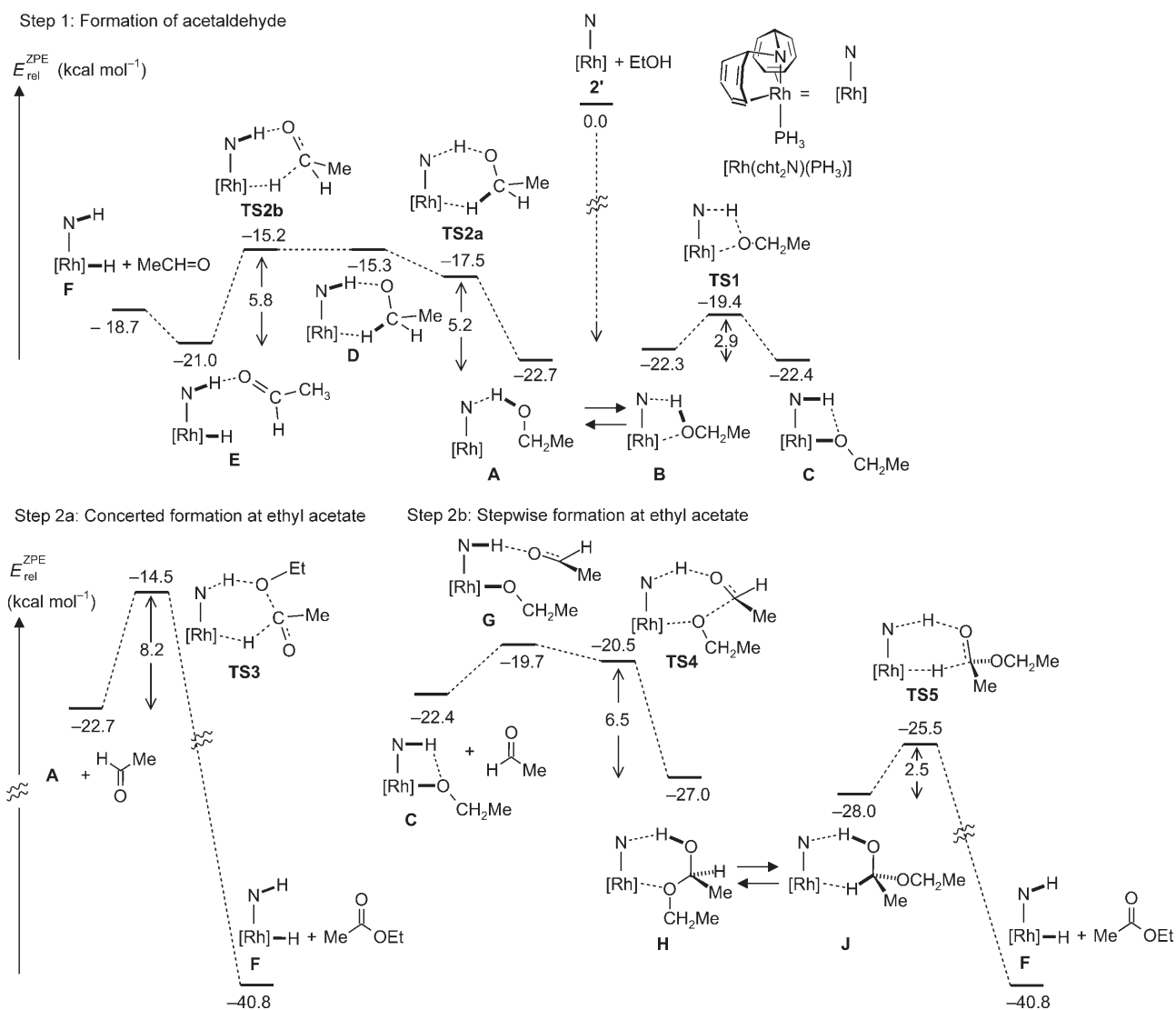
Figure 2. Formation of acetaldehyde (step 1) and ethyl acetate (step 2a or 2b) catalyzed by rhodium amide [\text{Rh}(\text{cht}_2\text{N})(\text{PH}_3)] ( 2' ) according to DFT calculations.
