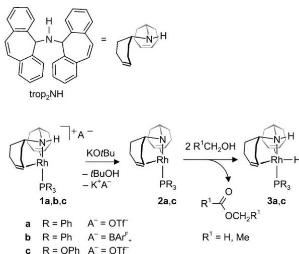
Scheme 1. Synthesis of amino olefin complexes 1a–c , the corresponding amido complexes 2a,c and their reaction with methanol or ethanol to give the amino hydride complexes 3a,c .
