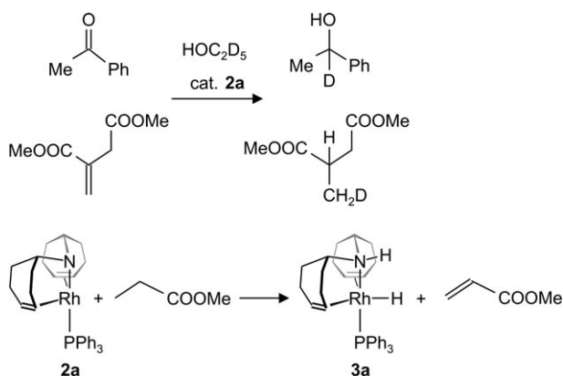
Scheme 3. Selective deuterium incorporation into acetophenone and itaconic acid dimethyl ester and dehydrogenation of propionic acid methyl ester promoted by 2a .
